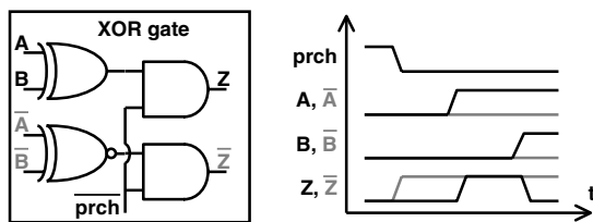
Fig. 2. SDDL: XOR-gate (left); timing diagram (right)
