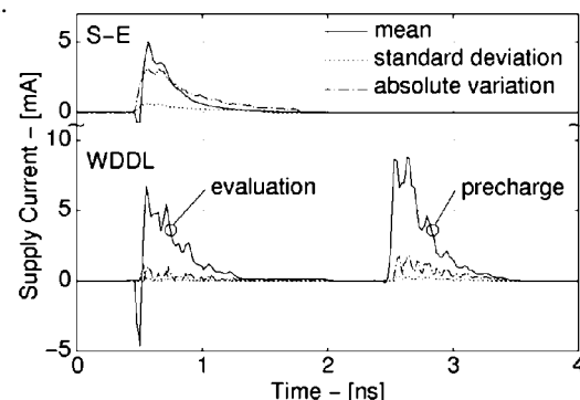
Fig. 9. Supply current characteristics
