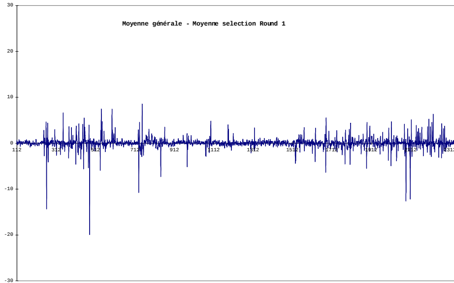
Fig. 2. An example of difference of the curves MC and MC' when the 6 bits are false
