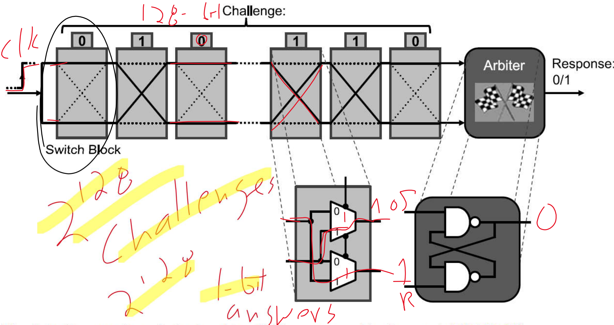
Fig. 2.1 Construction of a basic arbiter PUF as proposed by Lee et al. [43, 75, 78]
