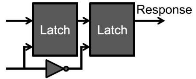
(b) D flip-flop PUF cell
